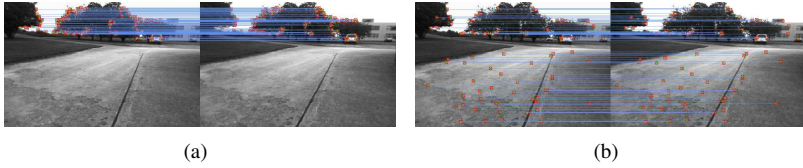
Figure 5: Quadrees provide a way to spread features in the image. (a) Taking the strongest Harris scores might lead to poorly constrained estimates. (b) Using a quadtree, it is possible to obtain points that do not necessary have high Harris scores but provide strong constraints.
